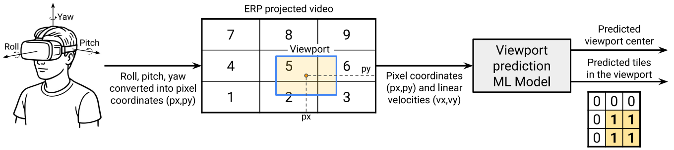
Fig. 1: Workflow for Viewport Prediction Using ML Models.
