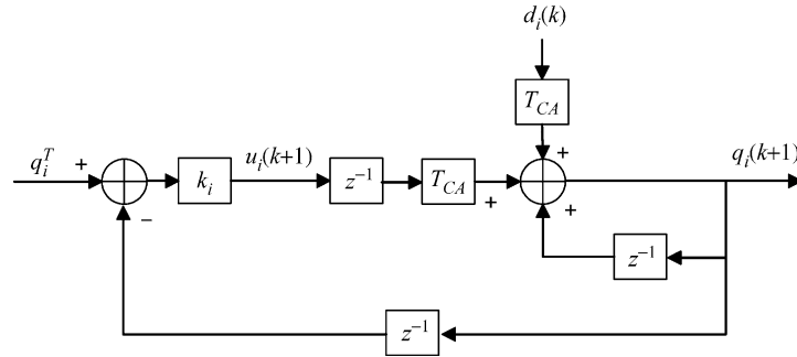
Fig. 3. HCCA-based closed-loop control scheme.
