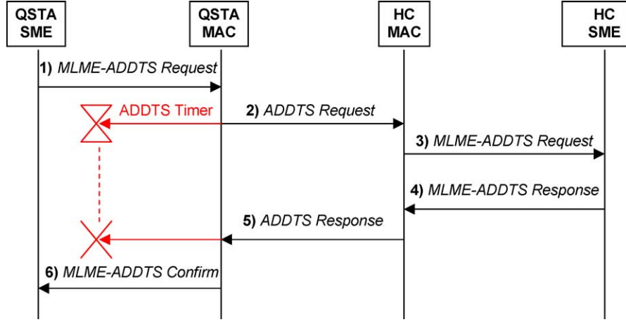
Fig. 2. Message Sequence Chart of Traffic Stream setup.
