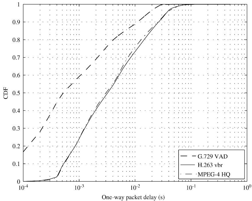
Fig. 8. CDF of the delay obtained using the proposed dynamic bandwidth allocation and CAC algorithms when \alpha=15 .
