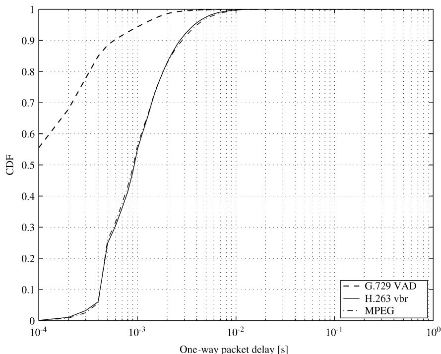
Fig. 5. CDF of the delay obtained using the simple scheduler and the standard CAC when \alpha=5 .
