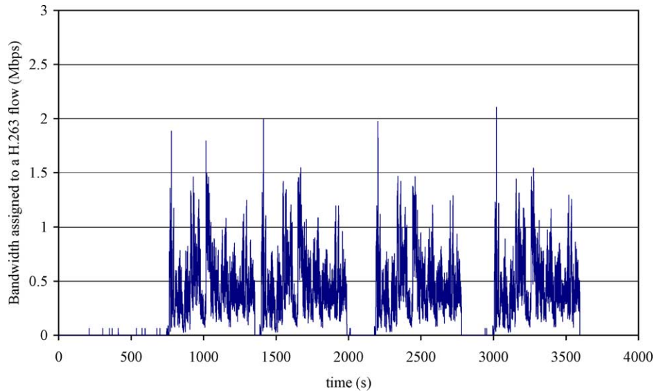
Fig. 10. Bandwidth assigned by the proposed algorithm to a H.263 flow when \alpha = 15 .
