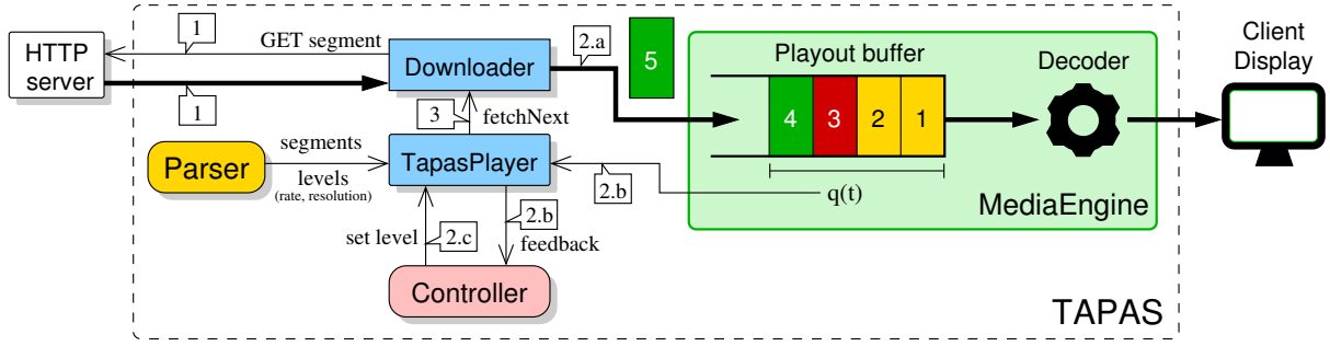
Figure 2: TAPAS workflow
