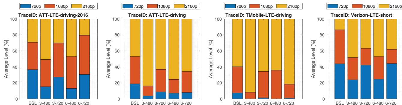
FIGURE 3 Breakdown of obtained video levels for each considered network trace
