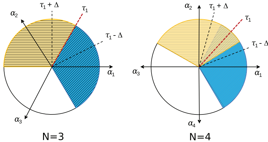
FIGURE 2 View selection algorithm in the case of N = 3 or N = 4 views
