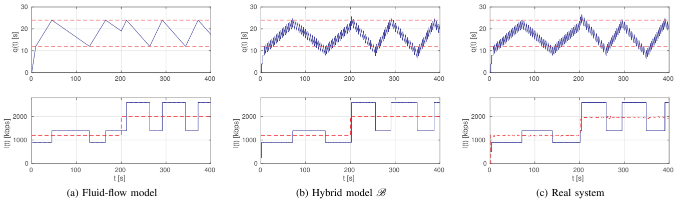
Fig. 6: Dynamics of the system with the Hysteresis controller and bandwidth increase from 1200 kbps to 2000 kbps
