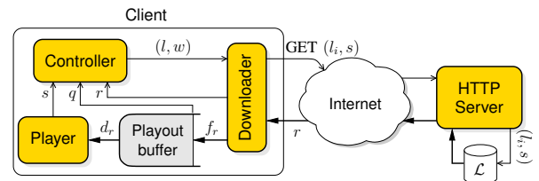
Fig. 1: An adaptive video streaming system
