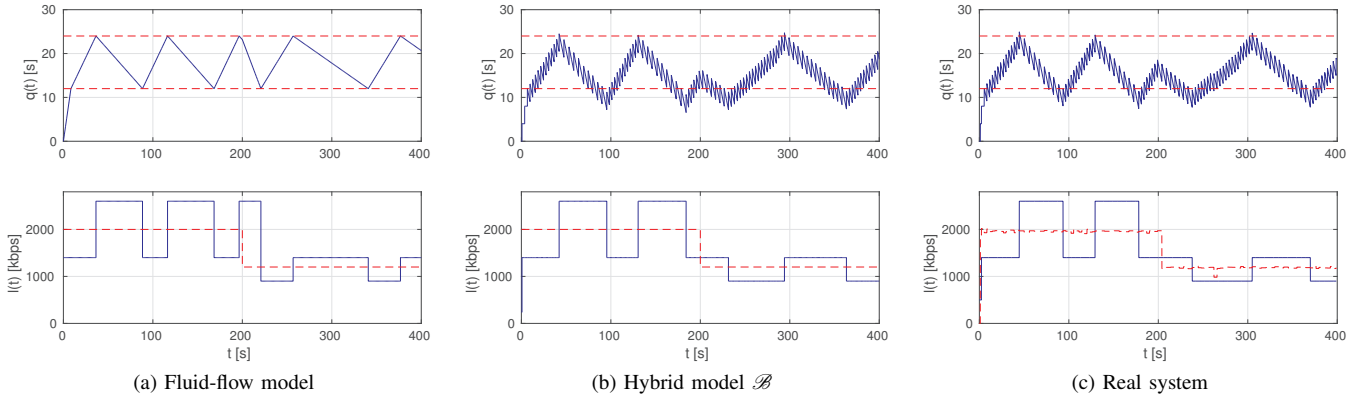
Fig. 5: Dynamics of the system with the Hysteresis controller and bandwidth drop from 2000 kbps to 1200 kbps
