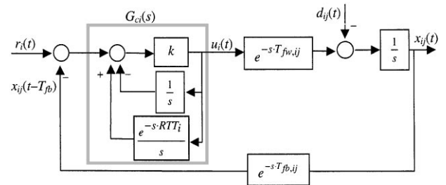
Fig. 3. Block diagram of the dynamics of the controlled bottleneck queue.
