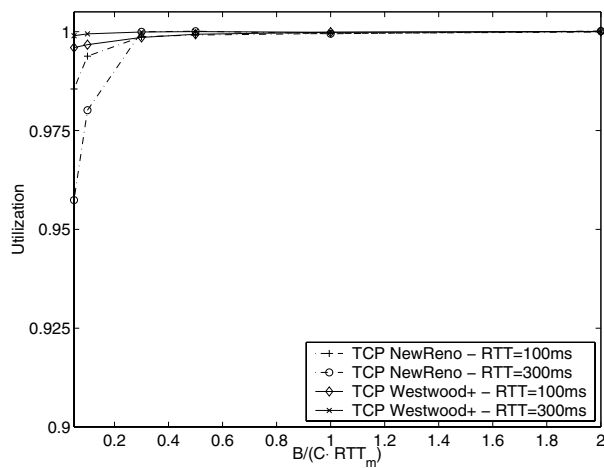
Fig. 8. Link utilization in a 200 fbs scenario with C=200\text{Mbit/s} as a function of the bottleneck buffer size.
