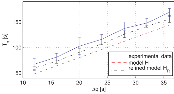
Fig. 8. Switching period T_s obtained through numerical simulations and network experiments as a function of \Delta q .
