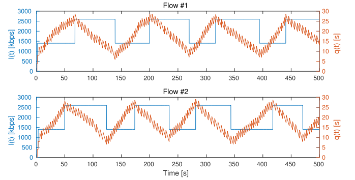
Fig. 9. Two video flows sharing a bottleneck with capacity C = 4 Mbps.
