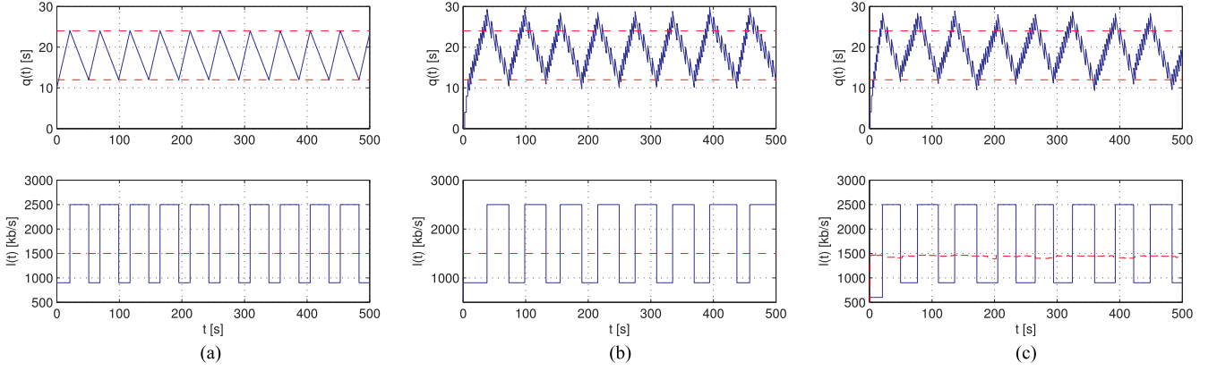
Fig. 7. Dynamics of q(t) and l(t) obtained through numerical simulations and network experiments. (a) Hybrid model \mathcal{H} . (b) Refined hybrid model \mathcal{H}_R . (c) Real system.
