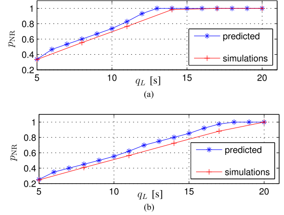
Fig. 11. No rebuffering probability p_{\text{NR}} function of q_L . (a) X = 15 s. (b) X = 20 s.
