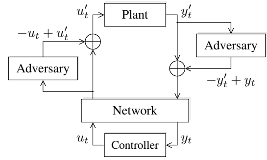
Fig. 1: Representation of a cyber-physical attack against a networked control system.
