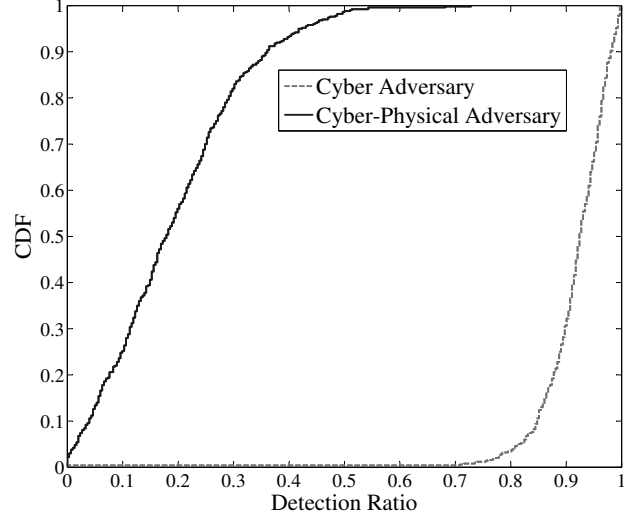
Fig. 2: Cumulative distribution function (CDF) of the detection ratio associated to the \chi^2 detector (see Section III-B), obtained by measuring the DR metric (see Equation 9) for 500 simulations (both cyber and cyber-physical adversary cases).
