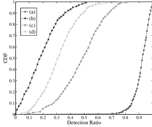
Fig. 4: Confronting the performance of the two detectors. (a) \chi^2 detector in [2], [3], and cyber adversary. (b) \chi^2 detector and cyber-physical adversary. (c) Multi-watermark detector with switching frequency set to 0.14Hz, and cyber-physical adversary. (d) Multi-watermark detector with switching frequency set to 0.05Hz, and cyber-physical adversary.
