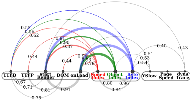
Figure 3: Pearson correlation between metric pairs.
