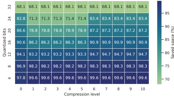
Figure 3: Saved space percentage using Draco codec varying qb and cl parameters
