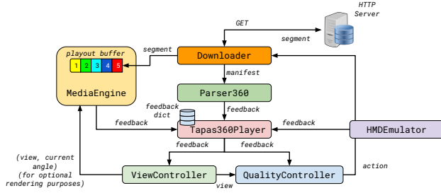
Figure 1: Workflow of the TAPAS-360° tool
