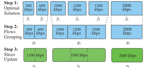
Fig. 5. The Quantized aggregation strategy.
