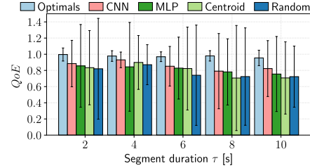
Fig. 6. Average QoE as function of the segment duration.
