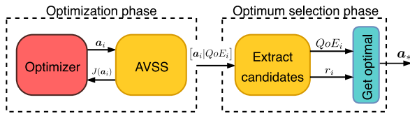
Fig. 3. Optimal computation procedure employed to build the ground truth dataset.
