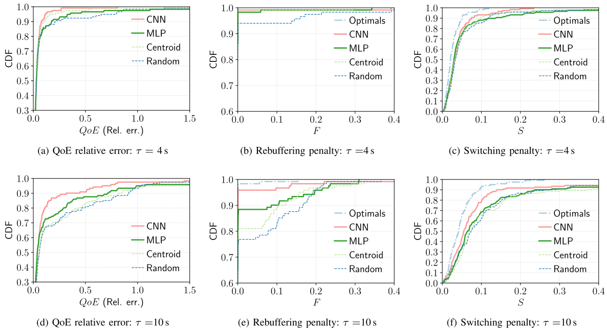
Fig. 7. Cumulative distribution functions of the QoE-related metrics in the case of videos with segment durations \tau equal to 4 s or 10 s.
