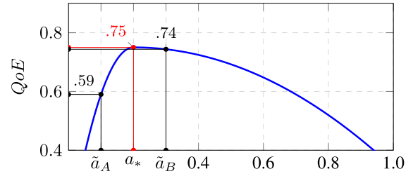
Fig. 5. Example of a one-dimensional reward mapping.
