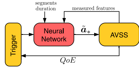
Fig. 2. ERUDITE architecture. A neural network acts as a supervisor and dynamically tunes the parameters of the AVSS controller to some values \tilde{a}_* to improve the QoE.
